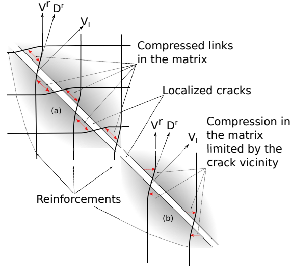
Figure 7.2: Compressed links in the matrix allowing dowel effect (a) or limiting dowel effect (b)
