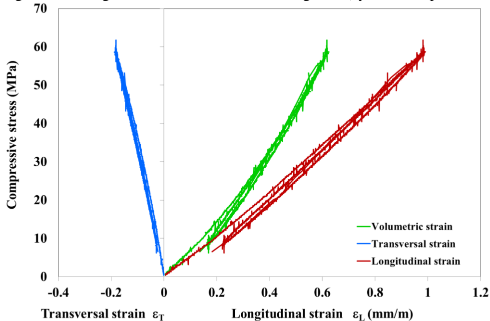
Fig.4 – Stress-strain curves with 3 loading-unloading cycles (specimen E)
