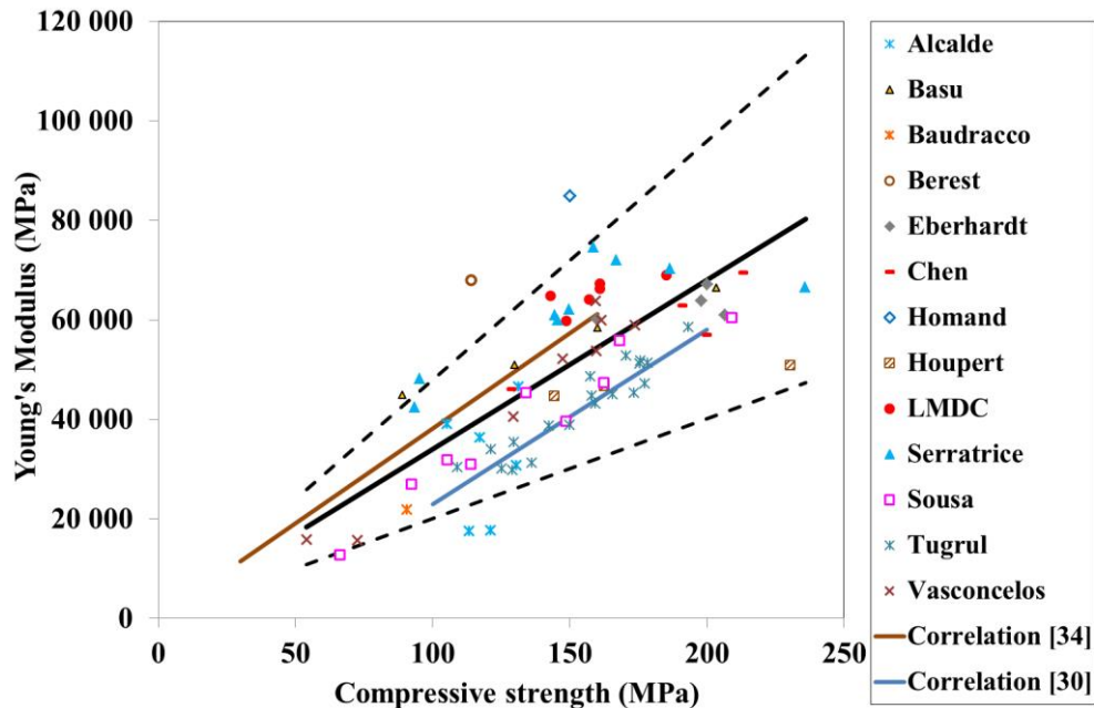
Fig.9. Young's modulus, E , versus compressive strength, f_c
