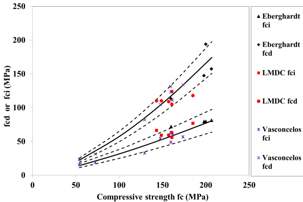
Fig.11 – Variation of f_{cd} and f_{ci} with the compressive strength f_c
