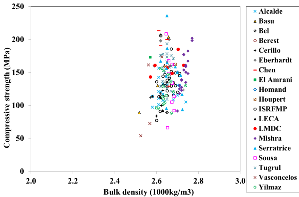
Fig.6. Compressive strength, f_c , versus bulk density, \rho
