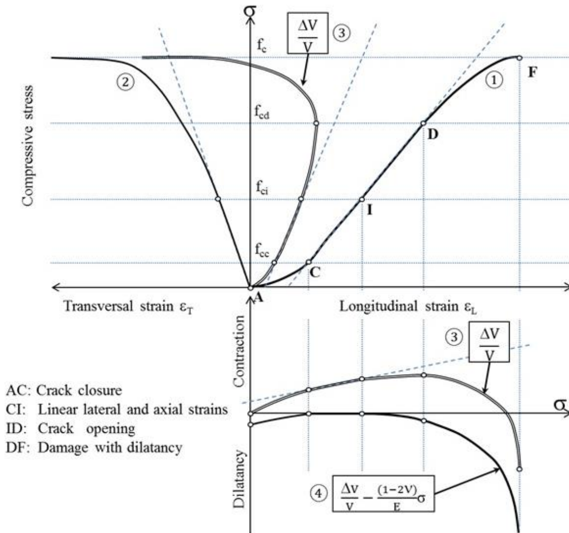
Fig.1 – Uniaxial compression test of granite. Typical stress/strain diagrams and changes in volume
