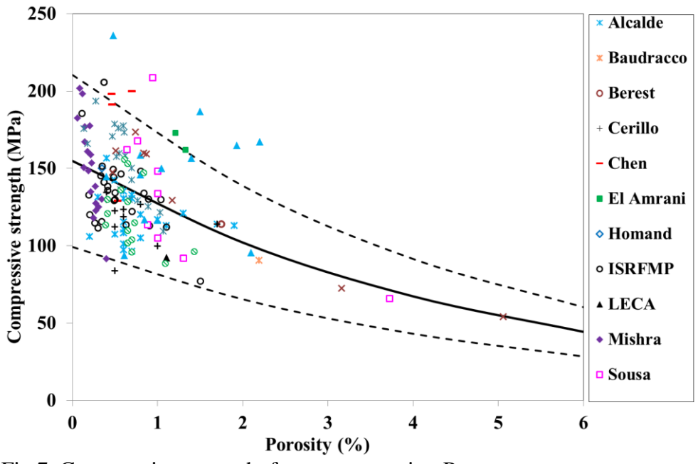
Fig.7. Compressive strength, f_c , versus porosity, P_o
