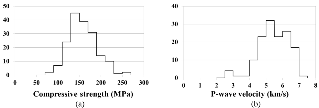
Fig.5. Histograms of compressive strength f_c (a) and ultrasonic P-wave velocity V_p (b)
