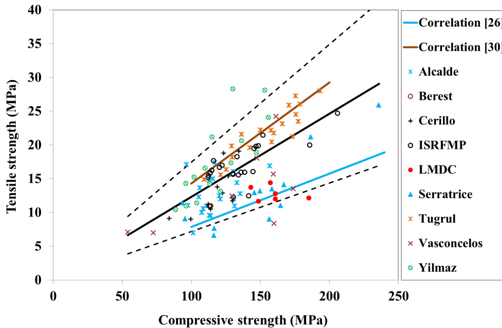
Fig.13. Tensile strength, f_{ct} , versus compressive strength, f_c .
