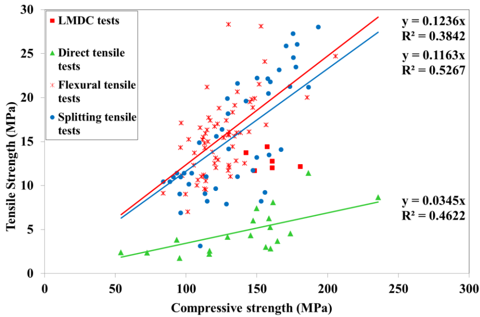
Fig.12. Tensile strength versus compressive strength, f_c , according to type of test
