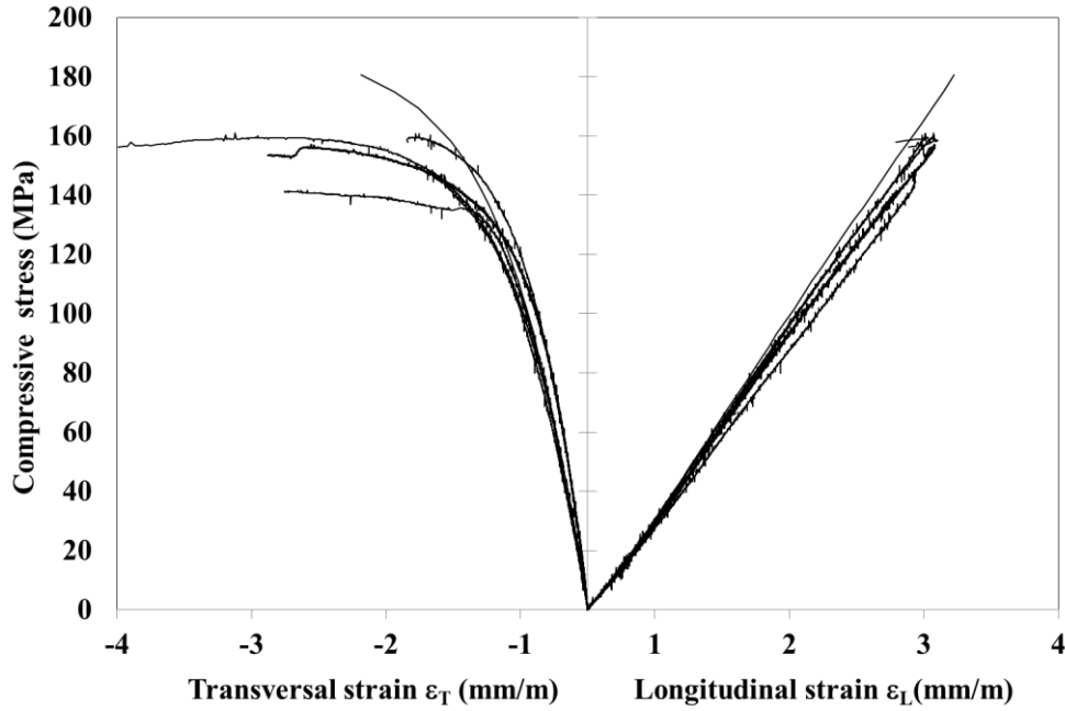
Fig.3 - Sidobre granite results. Stress-strain diagrams (cylindrical specimens 50 mm x 100 mm)
