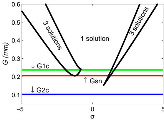
Fig. 5. Evolution of the multiplicity of periodic solutions for the system with parameters K = 3000 , \lambda_1 = 0.6 , \lambda_2 = 0.3 , \varepsilon = 0.01 .
