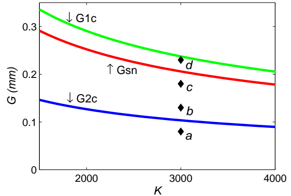
Fig. 6. Critical excitation amplitude as a function of the nonlinear stiffness, \lambda_1 = 0.6 , \lambda_2 = 0.3 , \varepsilon = 0.01 .
