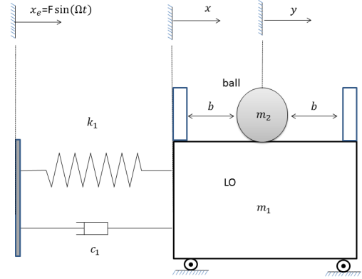
Fig. 1 Schema of a vibro-impact NES (impact damper)
