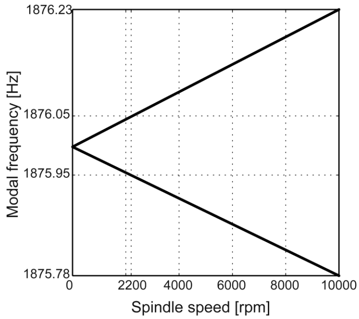
Fig. 8. Campbell diagram
