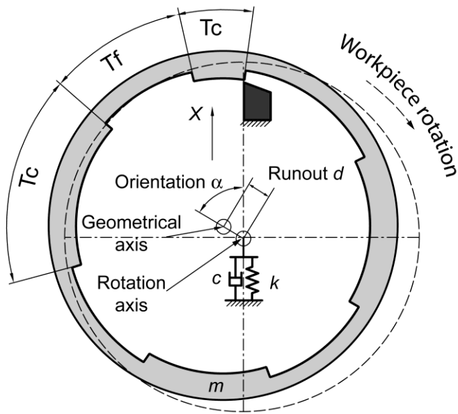
Fig. 9. Movement during mode coupling
