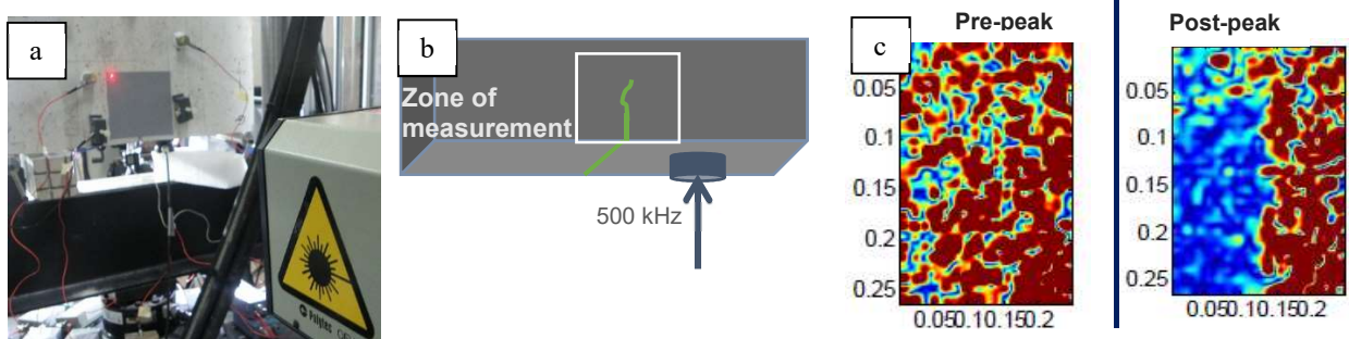
FIGURE 7. a) Us antenna measurement b) Principle c) Maps of diffused waves before and after the peak.
