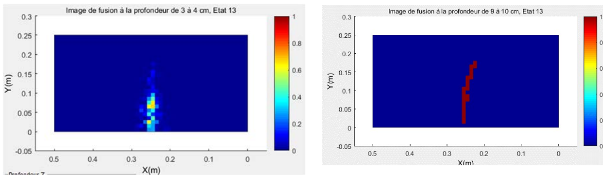
FIGURE 11. a) Hadamard Product of AE and Locadiff results b) DIC image for the same sample
