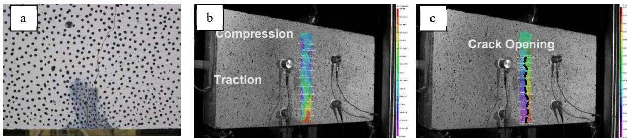
FIGURE 6. a) Speckle Pattern b) Strain distribution c) Crack way and opening
