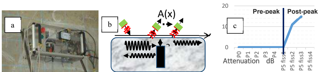
FIGURE 4. a) Ultrasonic surface waves scanner [20] b) Principle, c) Attenuation of the surface waves
