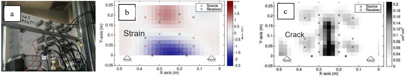
FIGURE 8. a) Transducers distribution b) Strain before the peak c) Crack propagation after the peak.
