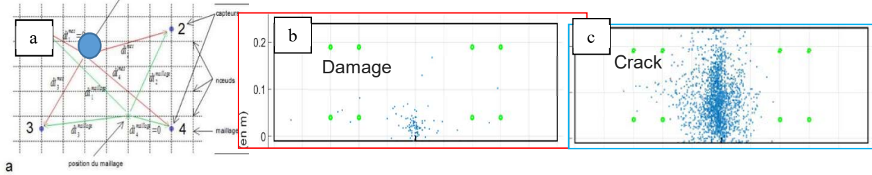
FIGURE 9. a) AE principle b) Events cumulation with damage before peak c) Events cumulation around the crack after peak
