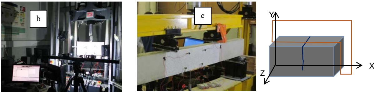
FIGURE 1. a) Follow-up testing of diffuse damage and its transition to continuous damage, b) Testing of crack opening and closure c) Sample for 3 points bending test with a crack.
