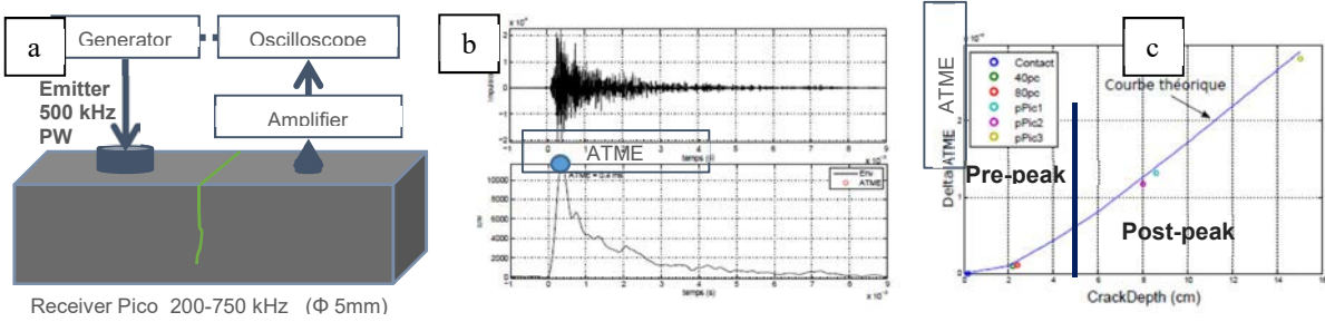
FIGURE 5. a) Diffused Waves analysis b) ATME c) Link between ATME and the crack depth
