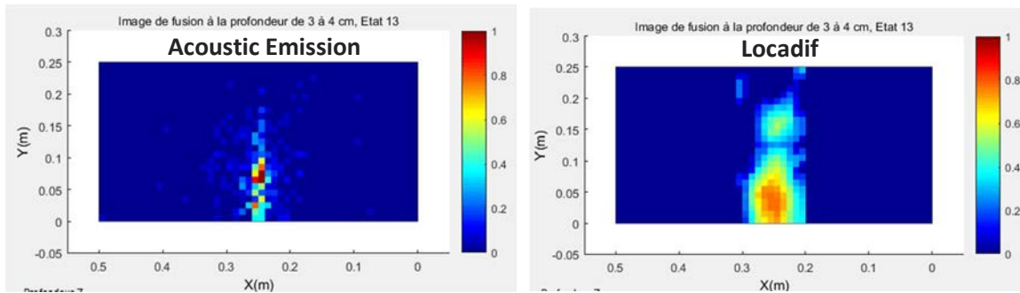
FIGURE 10. a) AE results for the mid-plan of the sample b) Locadiff results for the same plan.
