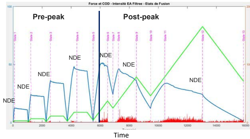
FIGURE 3. Loading cycle during the 3 point bending test. The blue line is the load, the green the crack mouth opening displacement (CMOD), the red corresponds to the events density of acoustic emission for each time.
