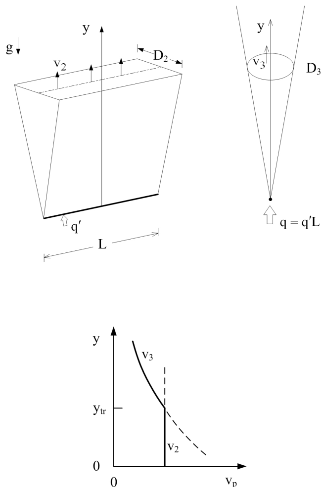
Figure 2 | Turbulent plumes, flat ( v_2 ) vs round ( v_3 ). The competition for more effective mixing (the smallest v ) dictates the transition from flat plume to round plume (and not from round to flat).
