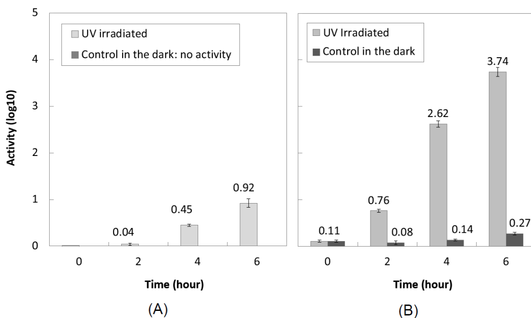
Figure 3. Antibacterial activity of TiO 2 as a support under UV irradiation (≈2.5 W/m 2 ): (A) standard conditions; (B) after application of a transparent plastic film on the inoculum. Mean ± SE, n = 3.
