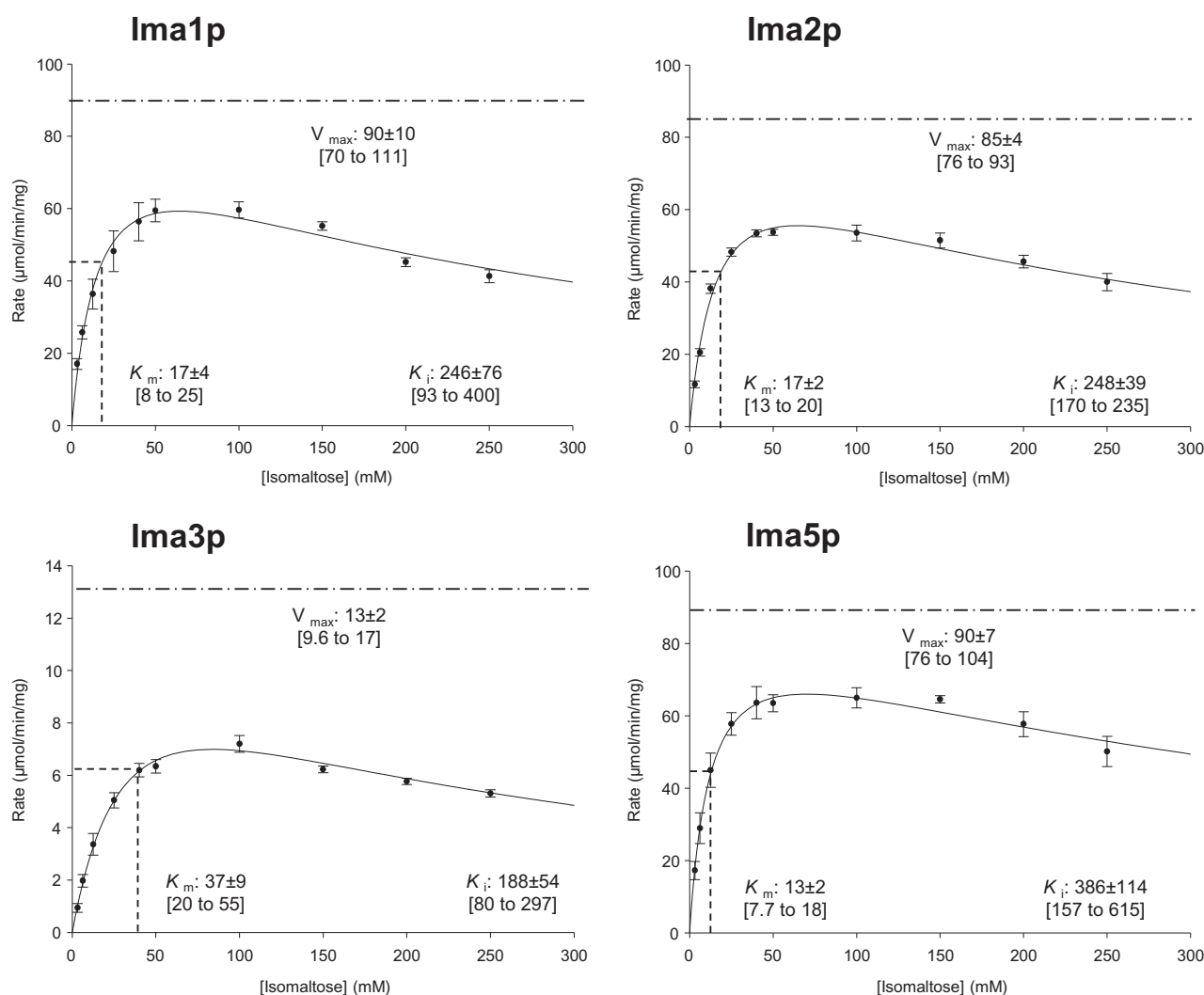
Fig. 1. Velocity–substrate profiles of Ima proteins for isomaltose. Non-linear curve fitting of the velocity as a function of substrate concentration, following the model v = (V_{\text{max}}S)/(K_m + S(1 + S/K_i)) with V_{\text{max}} : maximum velocity; S : substrate concentration; K_m : affinity constant and K_i : inhibition constant. Velocities were determined from an average of 5 independent assays. Estimated kinetic parameters, i.e. V_{\text{max}} (---), K_m (---) and K_i are expressed as the mean \pm SEM. The 95% confidence interval is given between brackets.
