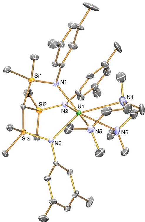
Fig. 4 Molecular structure of [U(Ts^{Xy})(pmdeta)] ( 2.pmdeta ) at 120 K with 40% probability ellipsoids. Hydrogen atoms and minor disorder components are omitted for clarity. Selected distances: 2.pmdeta - U1-N1 2.373(5), U1-N2 2.394(6), U1-N3 2.355(5), U1-N4 2.831(7), U1-N5 2.866(7), U1-N6 2.899(6) Å
