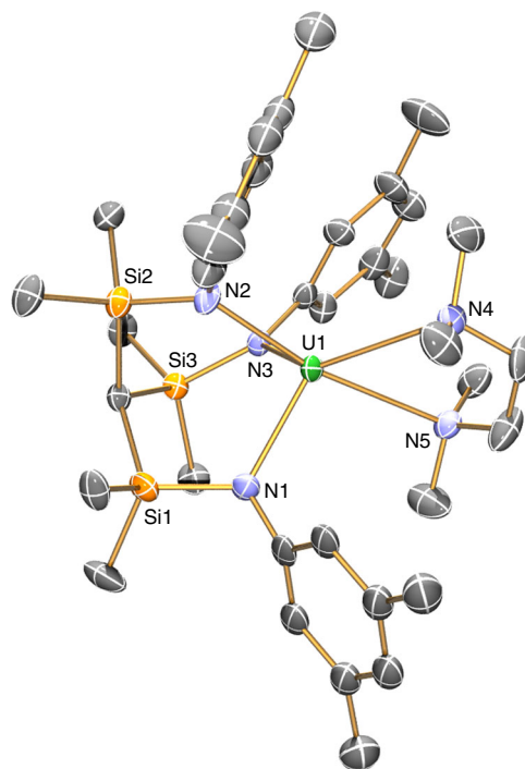
Fig. 3 Molecular structure of [\text{U}(\text{Ts}^{\text{Xy}})(\text{tmeda})] ( 2.tmeda ) at 120 K with 40% probability ellipsoids. Hydrogen atoms and minor disorder components are omitted for clarity. Selected distances: 2.tmeda -U1-N1 2.307(8), U1-N2 2.310(9), U1-N3 2.320(7), U1-N4 2.771(8), U1-N4A 2.760(7) Å
