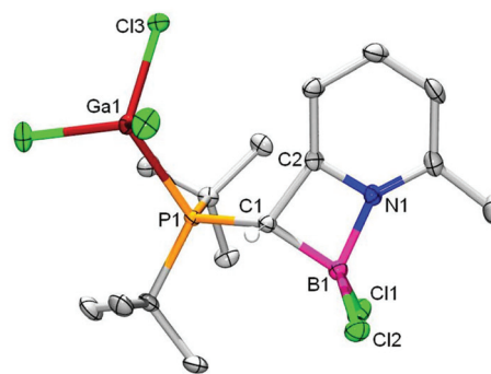
Fig. 5 Displacement ellipsoid plot (50% probability level) of 5-BCl 2 . Hydrogen atoms (apart from those on C1) are omitted for clarity. Selected bond lengths (Å) and angles (°): P1–C1 1.832(2); C1–C2 1.516(4); N1–C2 1.352(3); N1–B1 1.586(3); C1–B1 1.682(3); B1–C1 1.819(2); P1–Ga1 2.389(1); Ga1–Cl3 2.179(1); P1–C1–B1 132.2(2) (1); C2–C1–B1 84.4(2); C1–B1–N1 83.3(2); B1–N1–C2 93.9(2); N1–C2–C1 98.4(2); P1–C1–C2–N1–136.0.
