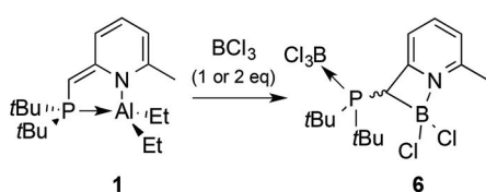
Scheme 7 Synthesis of 6 by transmetalation of 1 with 2 equiv. BCl 3 .
