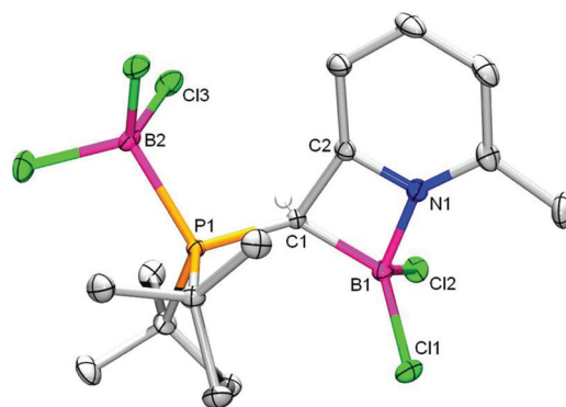
Fig. 6 Displacement ellipsoid plot (50% probability level) of 6 . Hydrogen atoms (apart from those on C1) are omitted for clarity. Selected bond lengths (Å) and angles (°): N1–B1 1.5805(25); B1–C1 1.6841(26); P1–B2 2.0441(21); C1–C2 1.5188(25); B1–Cl1 1.8220(21); B1–Cl2 1.8481(22); P1–C1 1.8419(19); N1–B1–C1 83.64(12); P1–C1–B1 133.05(13); N1–B1–Cl1 113.40(13); C1–P1–B2 105.87(8); P1–C1–C2–N1–135.23.
