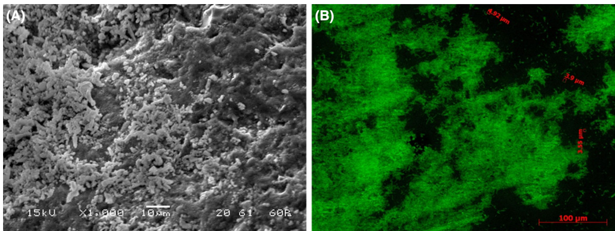
Fig. 8 Microscopic observation of the surface of solid matrices colonized by Hd (at pH 12, after 600 h of exposure): a SEM and b epifluorescence [131]
