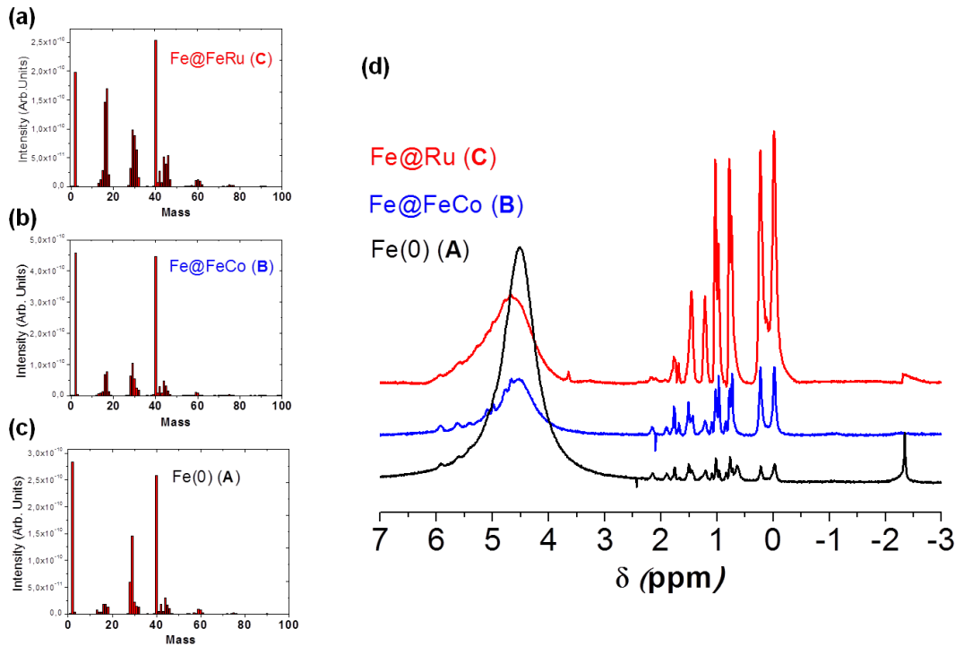
Figure 4: (a) mass spectra after FTS using (C); (b) mass spectra after FTS using (B); (c) mass spectra after FTS using (A) (d) 1 H gas NMR of the gas obtained after FTS using Fe(0) (A), Fe@FeCo (B) and Fe@Ru (C) as catalyst.
