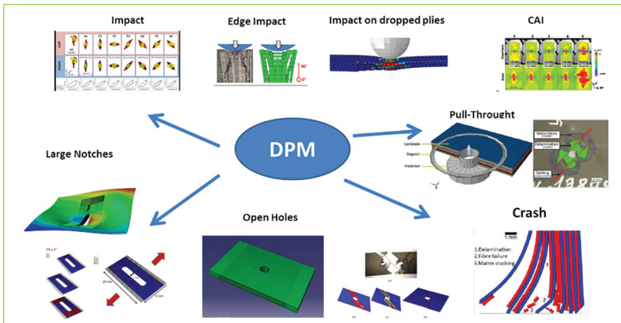
Fig. 9: DPM modelling
