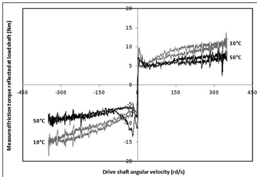
Figure 2. Measured friction torque reflected at output shaft for Harmonic Drive ® CPU-32-50-M reducer with standard grease (20 N m torque to load).
