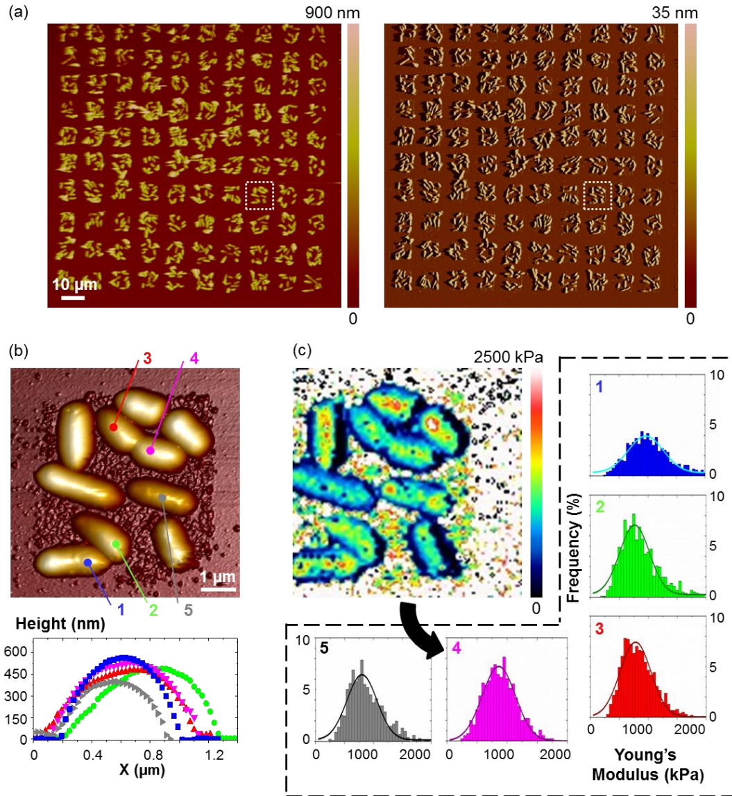
Figure 3. (a) AFM height image (left) and deflection error image (right) in buffer medium of Pseudomonas aeruginosa assembled on an array of 5\mu\text{m} square PEI patterns similar to the one presented in Fig. 2b, (b) deflection error image of ten Pseudomonas aeruginosa assembled on the square PEI pattern marked by a dashed square on (a), with height profiles of the five bacteria labelled on the deflection error image, (c) Young's modulus force volume mapping in buffer medium of the area observed in (b) with Young's modulus histograms of the five bacteria labelled in (b).
