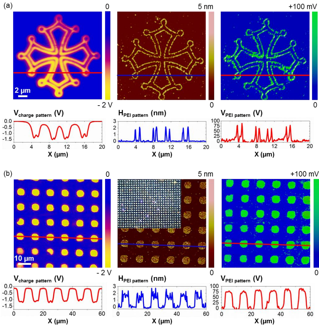
Figure 2. (a) Occitane cross-shaped PEI pattern fabricated by AFM nanoxerography and (b) array of 5 \mu\text{m} square PEI patterns fabricated by e- \mu CP nanoxerography. In each case, KFM surface potential images of the charge patterns written on a PMMA thin film are presented on the left panel, AFM height images and KFM images of the PEI patterns obtained after development are shown on the middle and the right panels respectively. Representative sections are systematically shown under each image. Note that a larger view by optical microscopy of the array of PEI squares is provided in inset of the AFM height image presented on the middle panel of (b).
