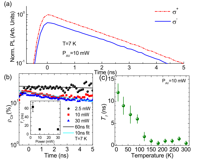
FIG. 6. (a) Temporal evolution of the polarization-resolved PL of Ge 0.95 Sn 0.05 at an average pump power P_{\text{AV}} of 10 mW and a lattice temperature of 7 K. Right-handed circular polarization ( \sigma^+ ) is shown as a dashed red line, whereas the left-handed helicity ( \sigma^- ) is reported as a blue line (the excitation laser is \sigma^+ polarized). (b) Low-temperature decay dynamics of the circular polarization degree \rho_{\text{circ}} . Black dots, red squares, and blue triangles refer to an average pump power equal to 2.5, 10, and 30 mW, respectively. The black (blue) line is a fit of the low (high) power decay curve which provides a decay time of 60 (10) ns. The inset demonstrates the derived spin relaxation time T_1 as a function of the excitation power. (c) Temperature dependence of T_1 for P_{\text{AV}} = 10 mW.
