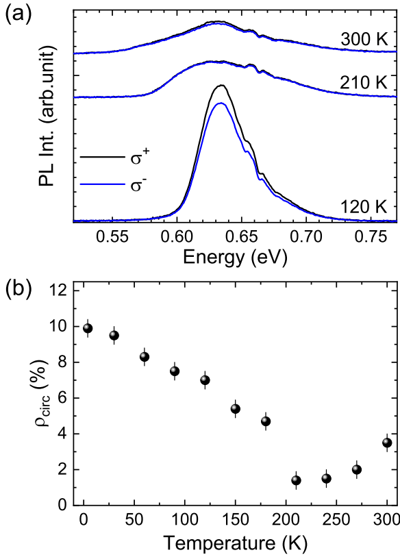
FIG. 5. (a) PL spectra for the Ge 0.95 Sn 0.05 /Ge/Si heterostructure measured at 120, 210, and 300 K for right- and left-handed circular polarizations, namely \sigma^+ (black curve) and \sigma^- (blue curve), respectively. The spectra have been vertically shifted for clarity. (b) Temperature dependence of the circular polarization degree ( \rho_{\text{circ}} ) measured under steady state conditions.
