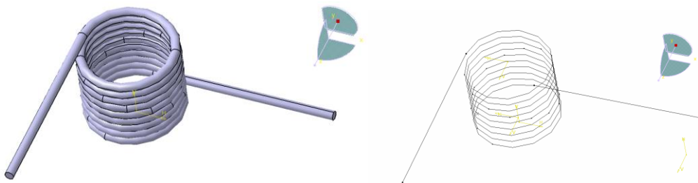
Figure 1. Example of a torsion spring with 3D and wire modelling
