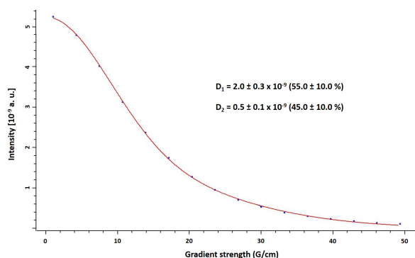
Fig. 3 Diffusional attenuation of the 1.90 - 2.20 ppm area for \text{Ru}_x(\text{CH}_3\text{COOH})_{0.4y} NPs dispersed in THF- d^8 at r.t. Data were analysed with a bi-exponential least-square fitting.
