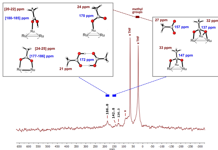
Fig. 6 ^{13}\text{C} CP Hahn-MAS NMR of \text{Ru}_x(\text{CH}_3\text{COOH})_{0.4y} NPs dispersed in mesoporous silica. DFT ^{13}\text{C} NMR chemical shifts of the acid group and carboxylate in various models. Blue: carboxyl group, burgundy: methyl group.
