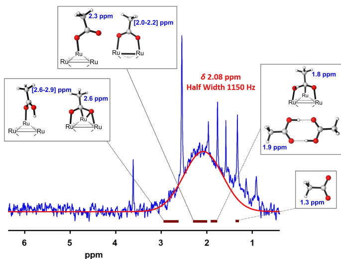
Fig. 2 Diffusion-filtered ^1\text{H} NMR spectrum of \text{Ru}_x(\text{CH}_3\text{COOH})_{0.4y} NPs dispersed in \text{THF-}d^8 at r.t. The broad signal at ca. 2.08 ppm was fitted with a Gaussian shape. The DFT ^1\text{H} NMR chemical shifts of the methyl group in various models ( (\text{CH}_3\text{COOH})_2 , \text{CH}_3\text{COO}^- , [\text{Ru}_6] clusters) are also given. The DFT results are summarized by the burgundy horizontal lines.
