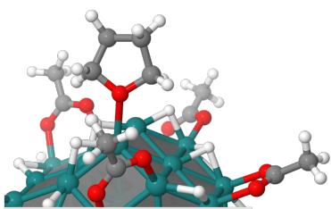
Fig. 9 Optimized geometry of Ru_{55}H_{32}(CH_3COO)_{15}(THF) .
