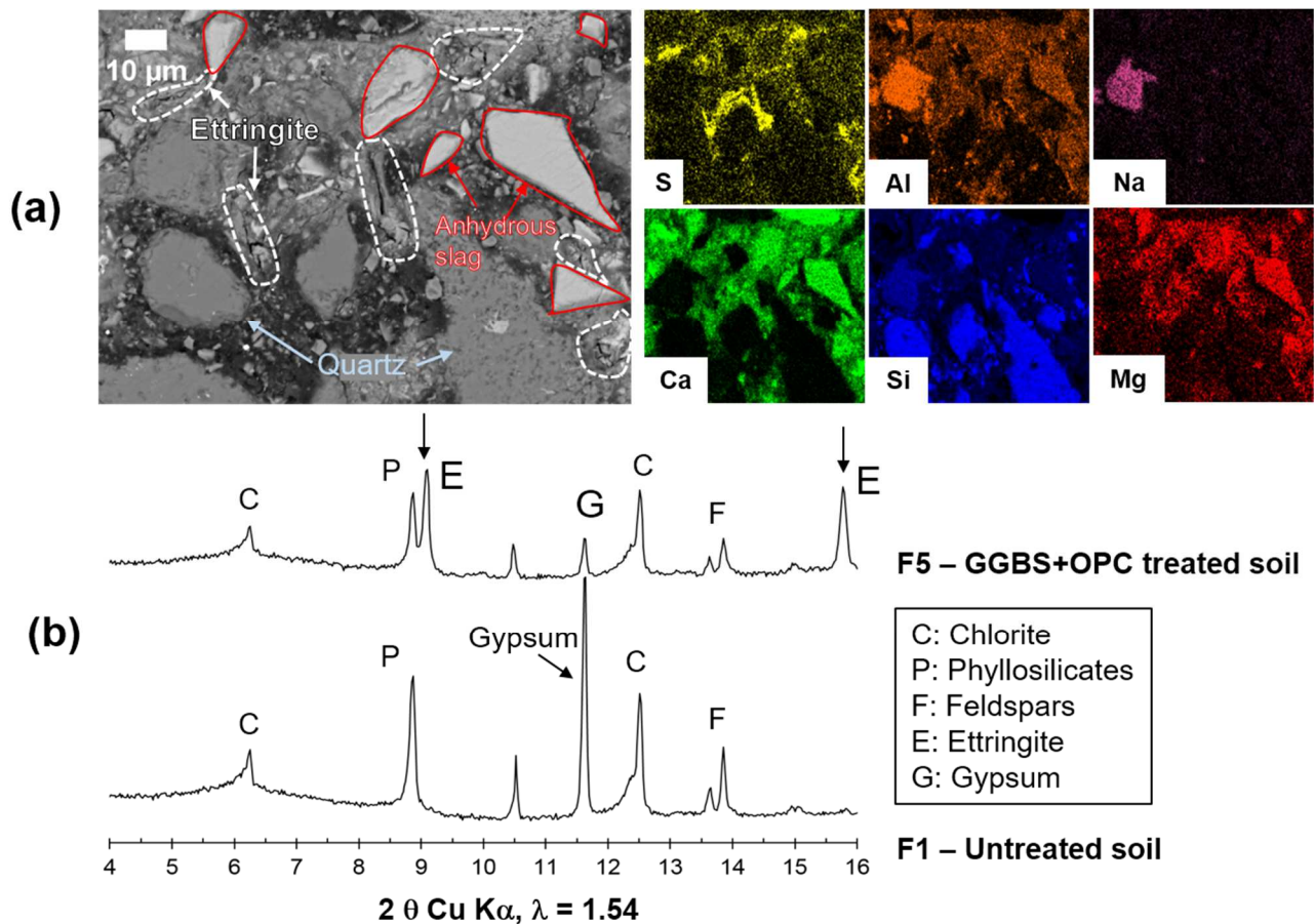
2 Figure 4 – Identification of ettringite in formulation F5 at 28 days of curing. (a) At left, BSE image of polished 3 section indicating the zones where ettringite phase was found. At right, EDS elemental mapping showing the 4 zonation of sulfur, calcium, aluminum, sodium, silicon and magnesium elements. (b) Selected range of the XRD 5 pattern obtained from formulation F1 (untreated soil) and formulation F5 showing the reduction of intensity of the 6 gypsum peak (G) and the appearance of ettringite peaks (E) in formulation F5.
