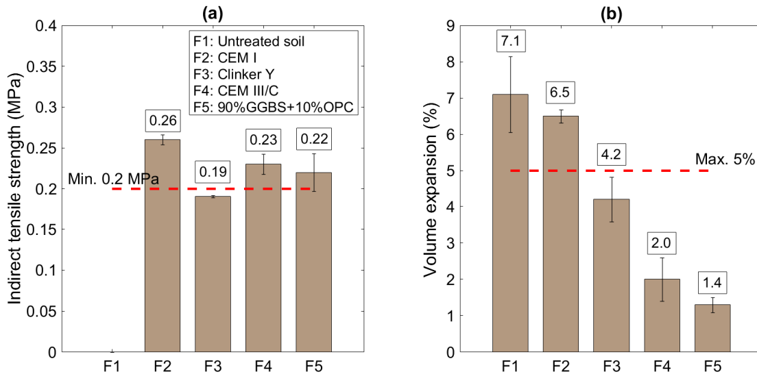
2 Figure 2 – Evaluation of mechanical properties and swelling for all formulations. The red dotted lines represent 3 the guideline established by French standard NF P 94-100. (a) Indirect tensile strength is expressed in MPa. (b) 4 Volume expansion is expressed in percentage.
