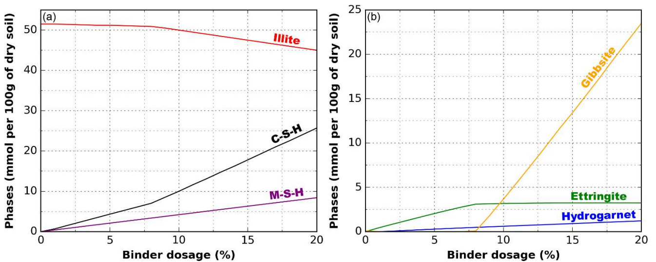
10 Figure 6 – Molar quantities of major phases calculated from the geochemical simulation of formulation F5 11 (90%GGBS+10%OPC) assuming a GGBS hydration level of 30%. All the data are plotted as a function of the 12 binder dosage. (a) Illite, C-S-H and M-S-H phases, (b) Ettringite, gibbsite and hydrogarnet.
