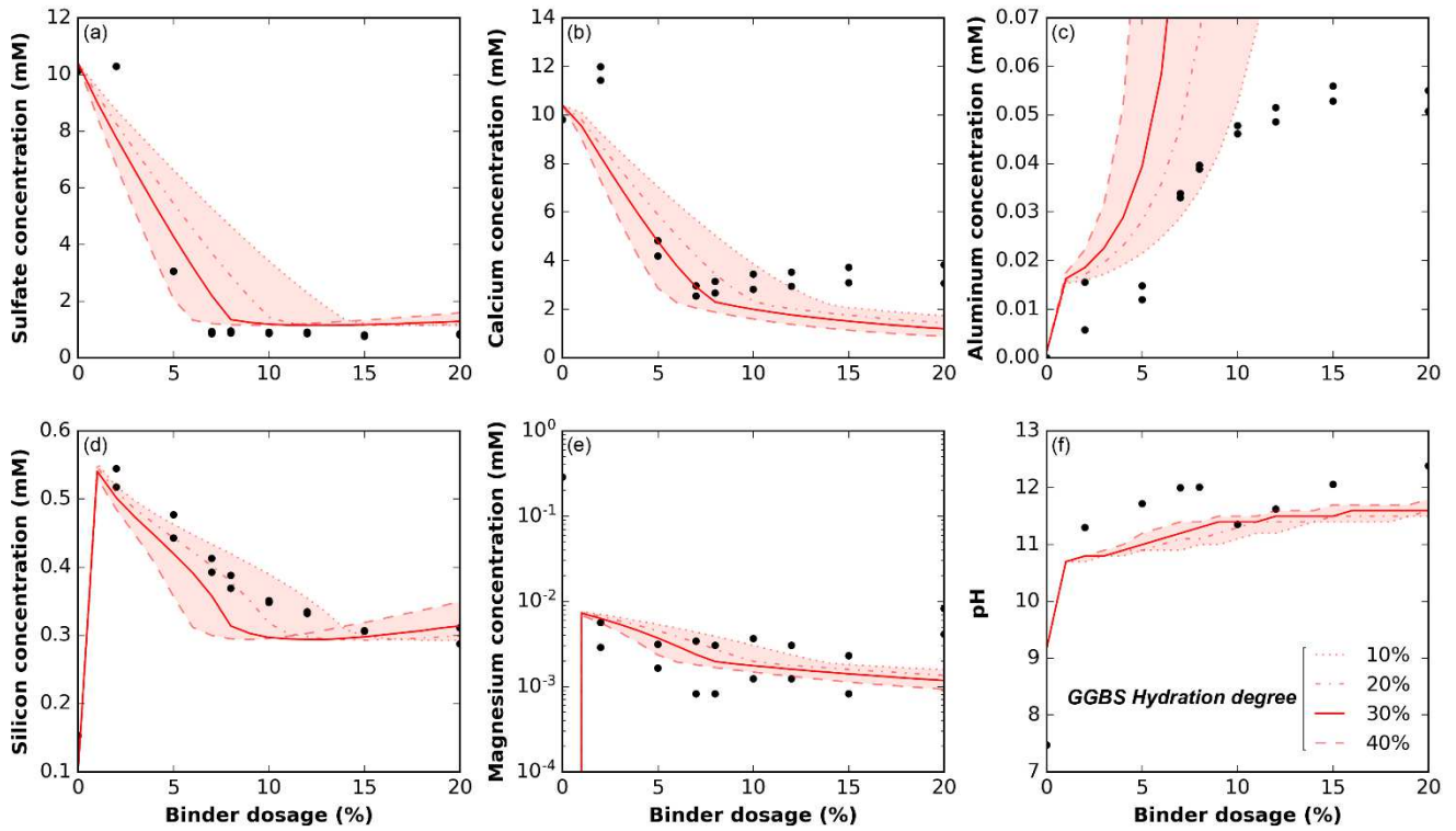
2 Figure 5 – Comparison between numerical and experimental data obtained from formulation F5 3 (90%GGBS+10%OPC). All the data are plotted as a function of the binder dosage. Black circles: experimental 4 data. Line with larger dots: 40% GGBS hydration level. Solid line: 30% GGBS hydration level. Line with smaller 5 dots: 20% and 10% GGBS hydration. (a) Leachable sulfate concentration, (b) leachable calcium concentration, 6 (c) leachable aluminum concentration, (d) leachable silicon concentration, (e) leachable magnesium 7 concentration (using a logarithmic scale), (f) pH values.
