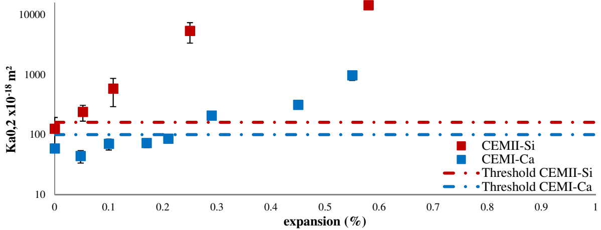
460 Figure 14: Evolution of apparent gas permeability coefficient according to the expansion for 461 concretes damaged by DEF
