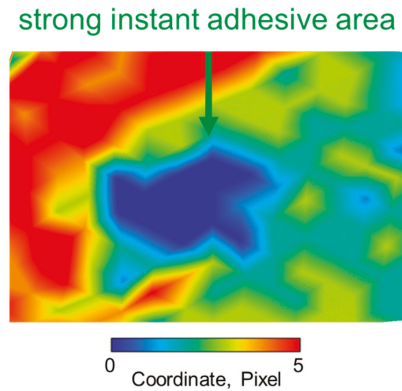
Figure 12. Displacement distribution region performed by SiDIC in the x-direction.
