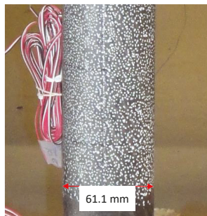
Figure 11. Random pattern on the surface of the thick composite tube [16].
