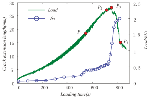
Figure 6. The curves of loading and crack extension length.
