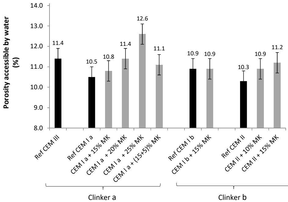
Figure 3 – Water porosity of concrete mixtures (28 days)
