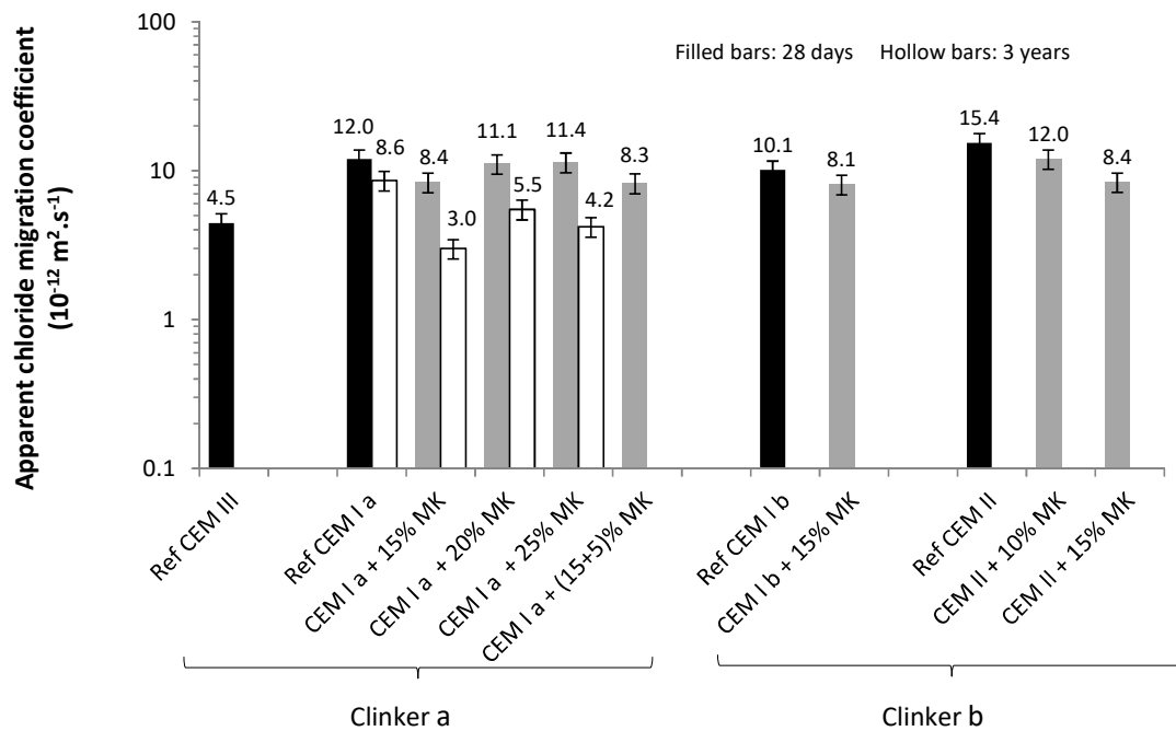
Figure 5 – Chloride migration coefficient of concrete mixtures (after 28 days and 3 years of curing)
