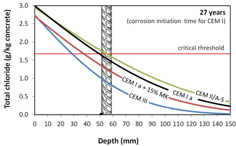
Figure 12 - Relation between quantity of chlorides and the chloride depth after 27 years of exposure (mixtures CEM I, CEM II/A-S, CEM I + 15 and CEM III/A)
