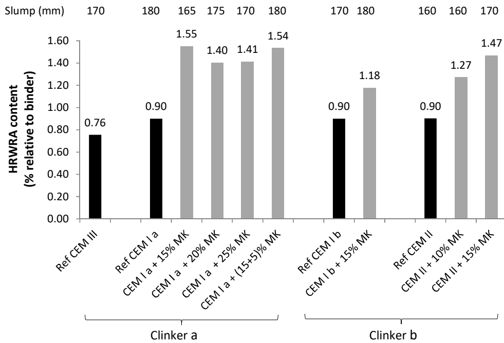
Figure 1 – HRWRA content (relative to binder) necessary to obtain a constant workability of concrete (except Ref CEM I with cement B, which had a lower slump).
