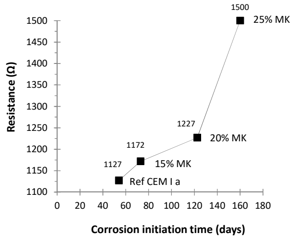
Figure 11 – Correlation between the resistance of the concretes (impedance tests) and the time necessary for corrosion to be initiated (accelerated corrosion test), for concretes based on CEM I with and without MK.
