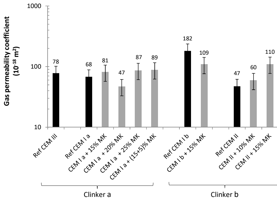
Figure 4 – Gas permeability of concrete mixtures (28 days)
