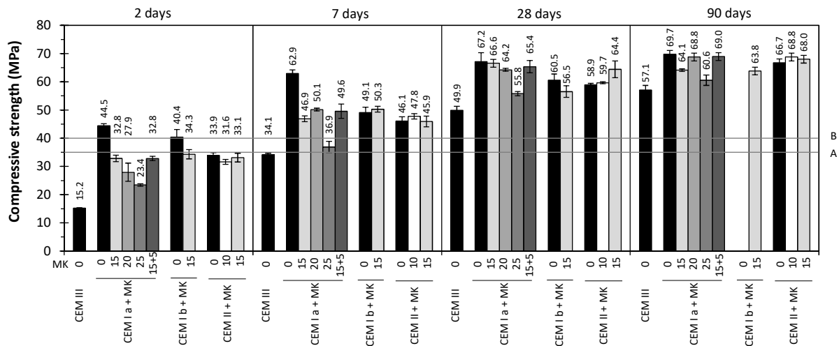
Figure 2 - Compressive strength of concrete mixtures between 2 and 90 days. A (35 MPa) is the minimum value of 28-day strength required for the XS3 exposure class, according to NF EN 206-1/CN. B is the design 28-day strength of the concrete mixtures.
