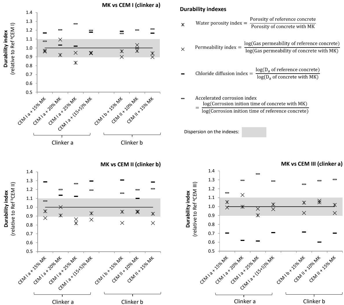
Figure 8 – Durability indexes defined as the ratios between concrete containing MK and reference concretes (CEM I, CEM II, CEM III)
