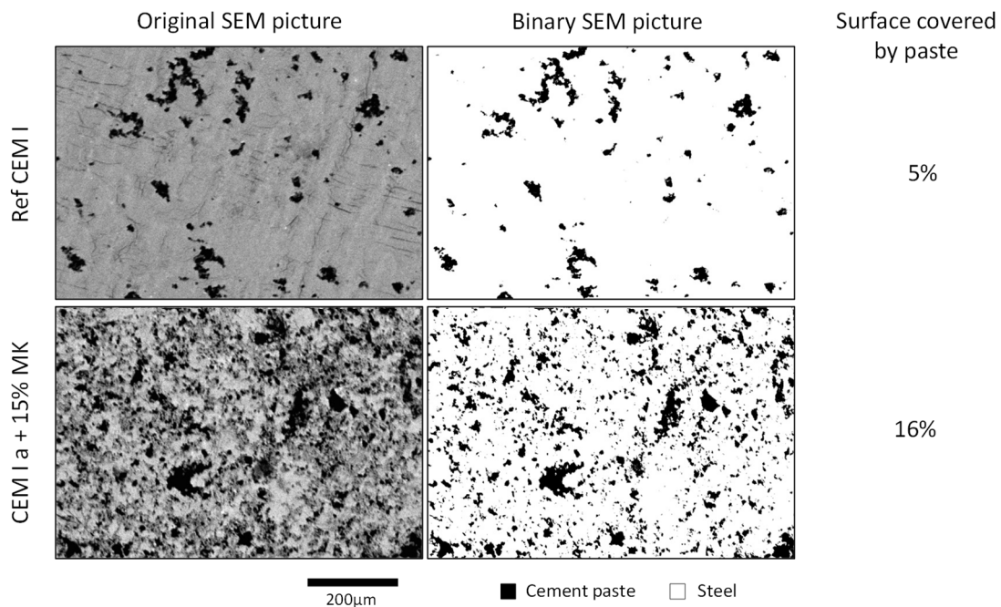
Figure 10 – SEM observations and surface quantification of the cement paste remaining on steel plates after the separation of the two materials. Cases of CEM I and CEM I + 15% MK.
