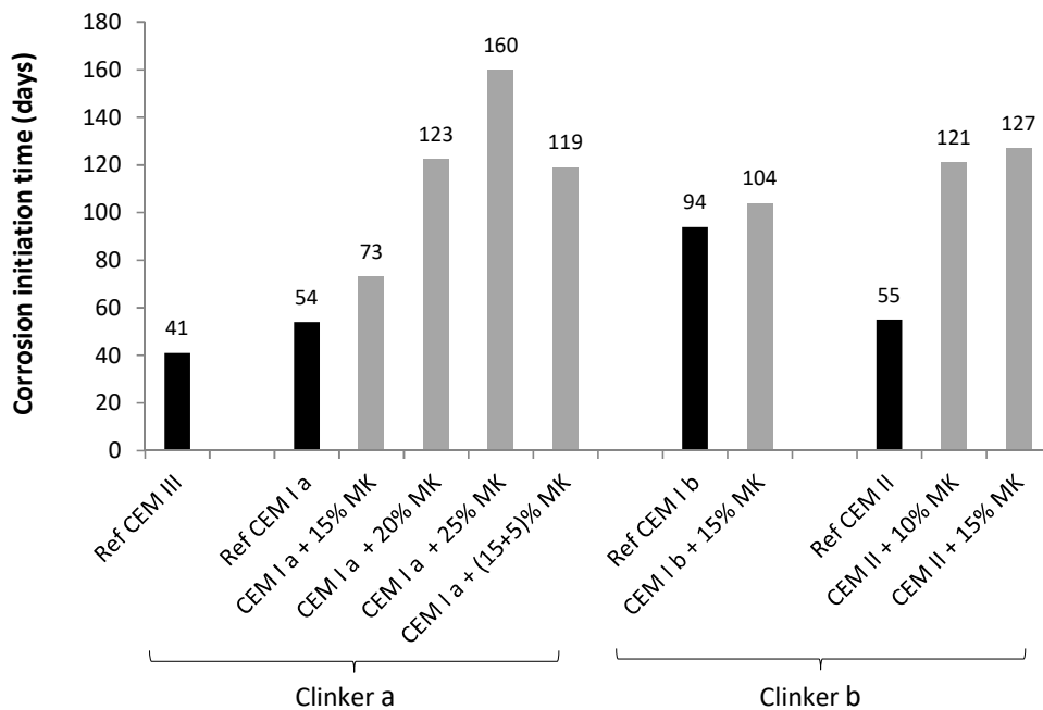
Figure 7 – Corrosion initiation time (accelerated tests) of concrete mixtures aged of 28 days
