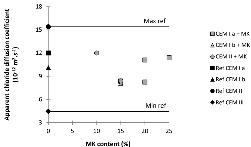
Figure 6 – Chloride migration coefficient of concrete mixtures versus MK content (28 days)
