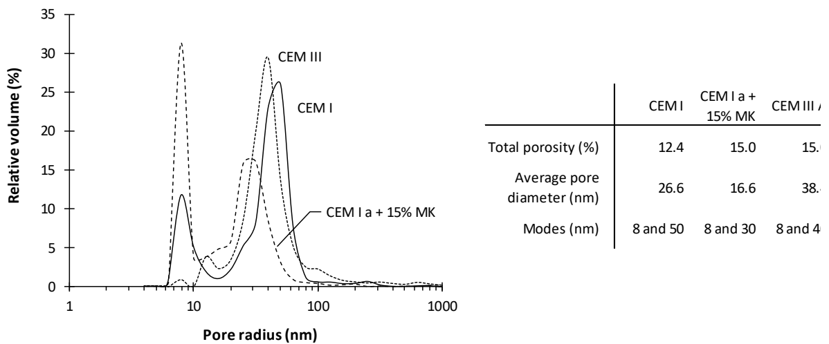
Figure 9 – Pore size distribution of cement pastes (CEM I, CEM I + 15% MK, CEM III) cured for 28 days, obtained by mercury intrusion porosimetry.
