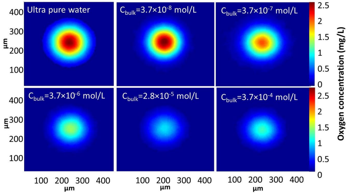
Figure 7: Oxygen concentration field in the wake of a bubble 0.33 seconds after the bubble's passage, in solutions containing different concentrations of TX100
