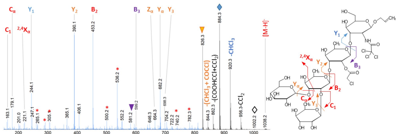
Figure 6. UHPLC-ESI-MS/MS spectrum of the pentasaccharide M40-4 isolated as [M-H]^- at m/z 1038.21 at t_R = 22.86 min in samples from M40 validated as being substituted at OH-3 B (P3'). The blue area of the spectrum is enlarged by a factor of 4 in the intensity axis. Annotations in red correspond to intact product ions. Annotations in blue correspond to product ions with a loss of CHCl_3 . Annotations in purple correspond to product ions with a loss of COCHCl . Annotations in orange correspond to product ions with a loss of CHCl_3 + COHCl . All these labile function losses are in agreement with the structure. Red * indicate consecutive fragmentations, \nabla indicate H_2O loss, \diamond indicate HCl loss. For clarity, only one fragment per pair (B, C and Y, Z) was reported on the annotated structure.
