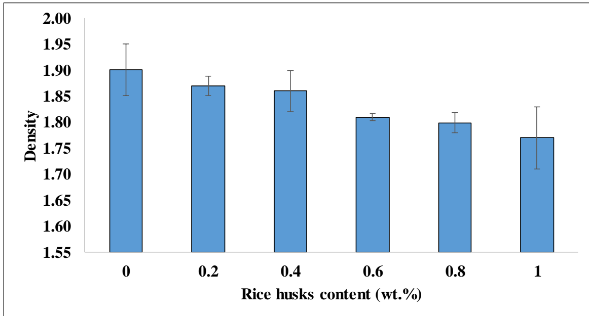
Figure 11: Density of adobes versus rice husk content
