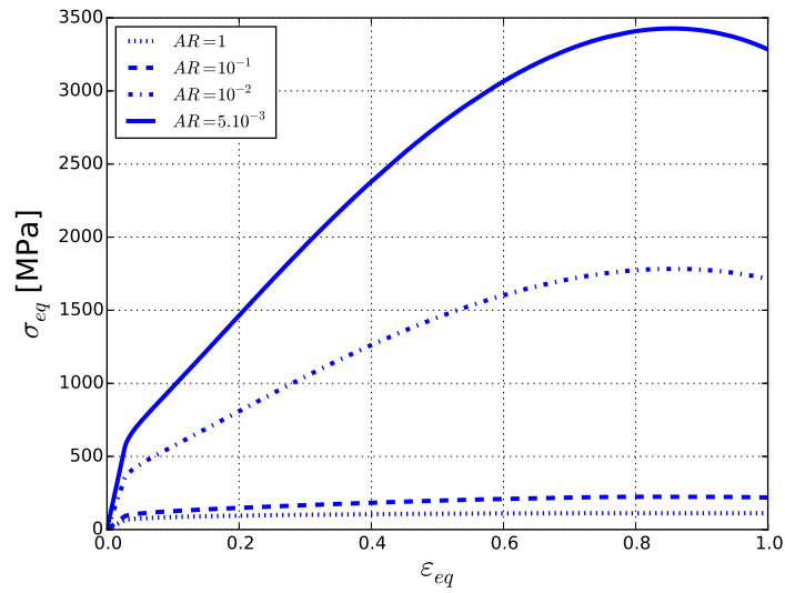
Figure 7: Aspect ratio variation of GPL/PA-6 composite for f_l = 0.1 and \alpha_0 = 0.3 .
