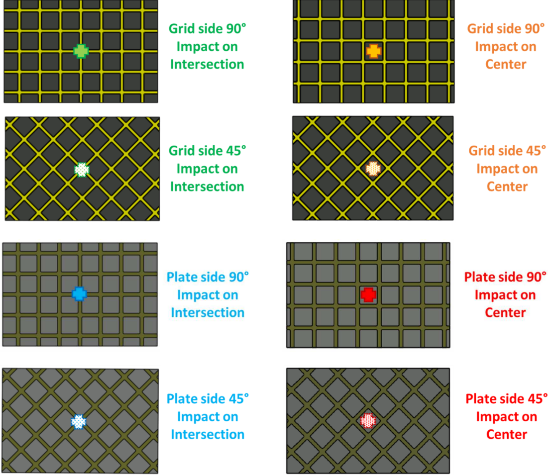
Figure 17. The 8 impact configurations.
