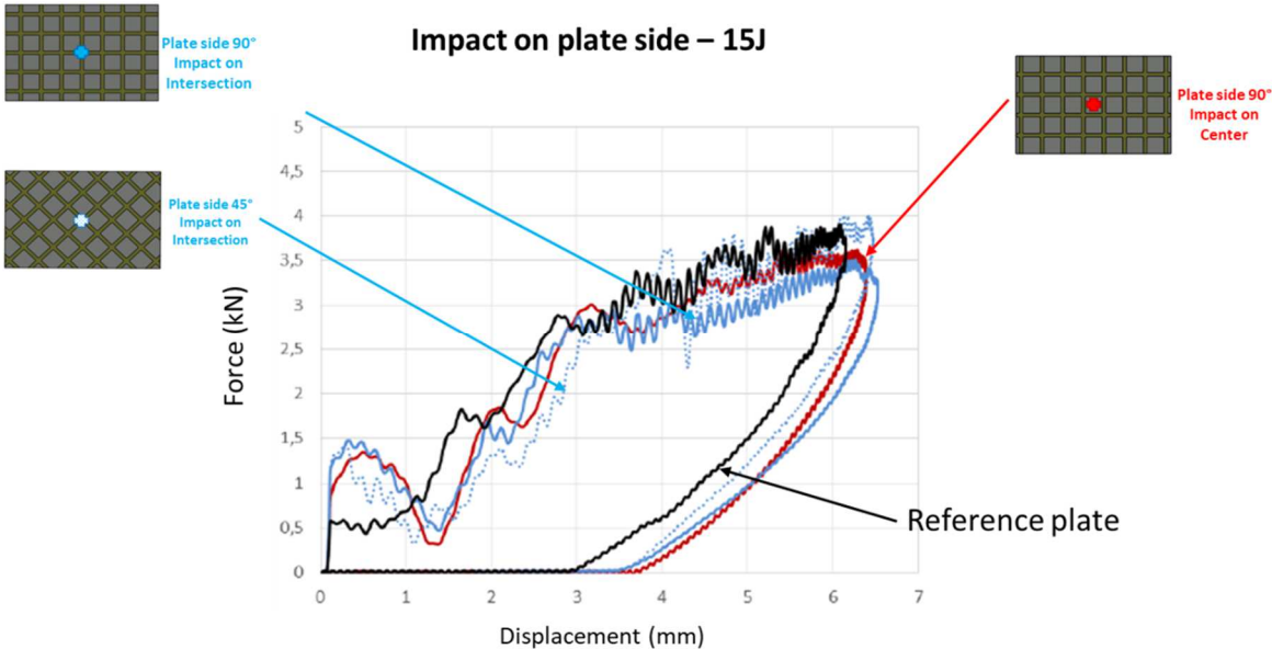
Figure 27. Displacement force curves for an impact at 15 J, plate side.
