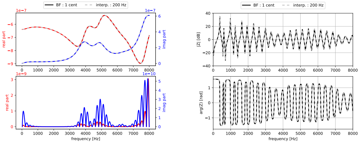
(a) Frequency behaviour of a randomly chosen matrix coefficient: upper graph shows real (red) and imaginary (blue) parts with respect to the frequency; lower graph shows absolute error between the approaches.
