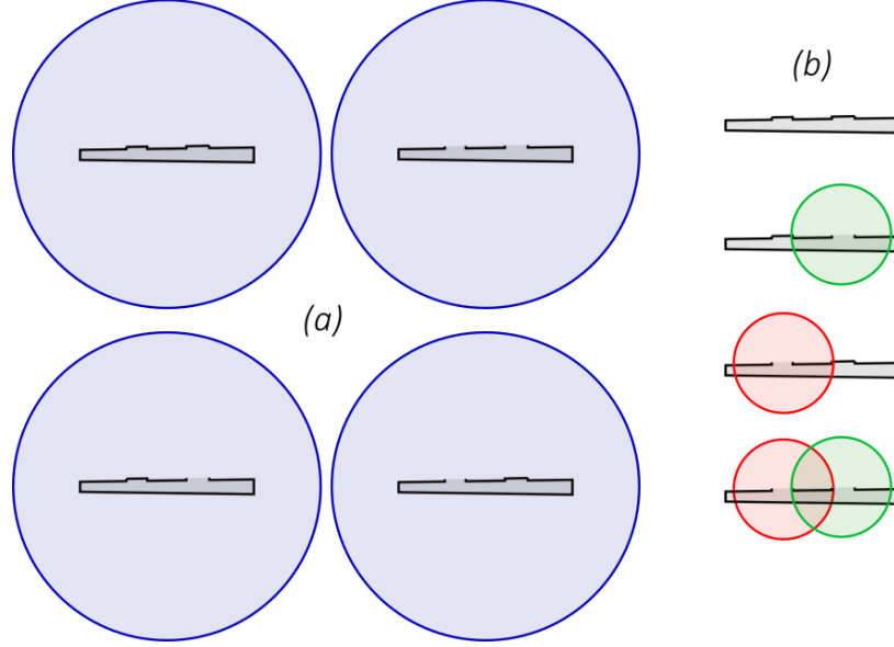
Figure 2: Sketch of the partitioned modelling strategy using blind spheres using H = 2 holes and N_f = 4 fingerings. The naive strategy (a) required 4 large spheres to model exterior domain, whereas the partition domain requires only 2 small blind spheres which can be activated or not depending on the fingering considered.
