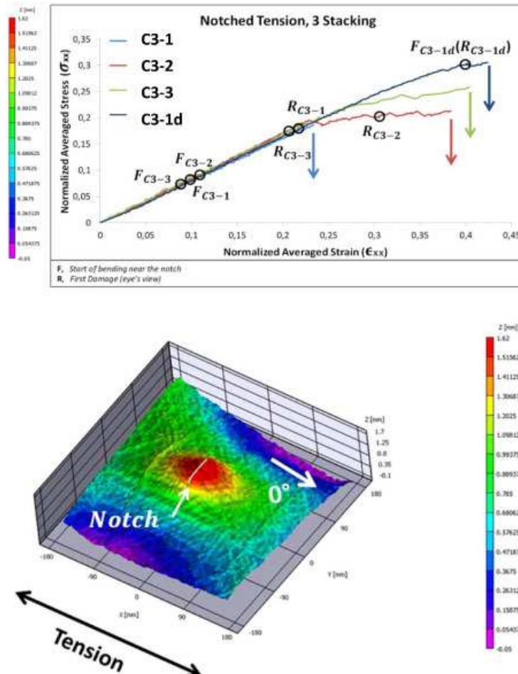
Figure 9. Influence of the stacking sequence and thickness on the notched tensile behavior, (b) Bending around the notch - FC3 – 1 for C3-1 stacking sequence.
