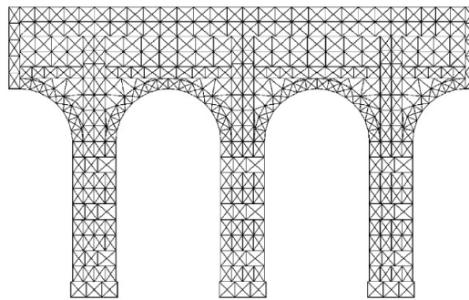
Fig. 19. UDEC internal finite element mesh.
